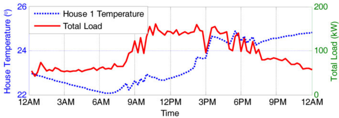
(a) Autonomous temperature control
